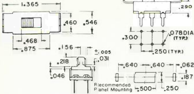
FIGURE 8. DOUBLE POLE, DOUBLE THROW - TWIST TAB
