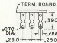
TERMINALS (.020 Thick)
